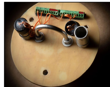
Figure 9-3: End Cap/Bulkplate
