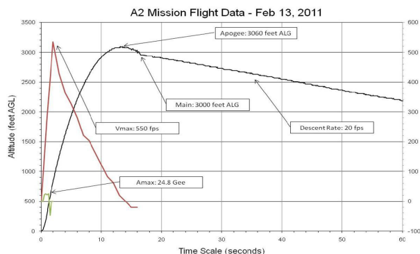
Figure 6-6: Plotted Trajectory Data from Commercial Software Package
