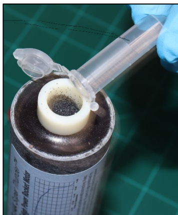
Figure 14-8: Pour Black Powder into Deployment Well
