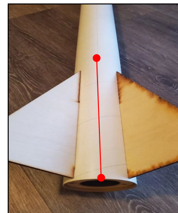
Figure 13-25: Measuring Fin Slots (Top); Measuring Half Way between Two Fin Slots (Top Center); Drawing a Line at the Half Way Mark on Tape (Center); Drawing the Half Way Mark on the Air Frame (Bottom Center); Markers to Indicate Rail Button Placement/Alignment (Bottom)
