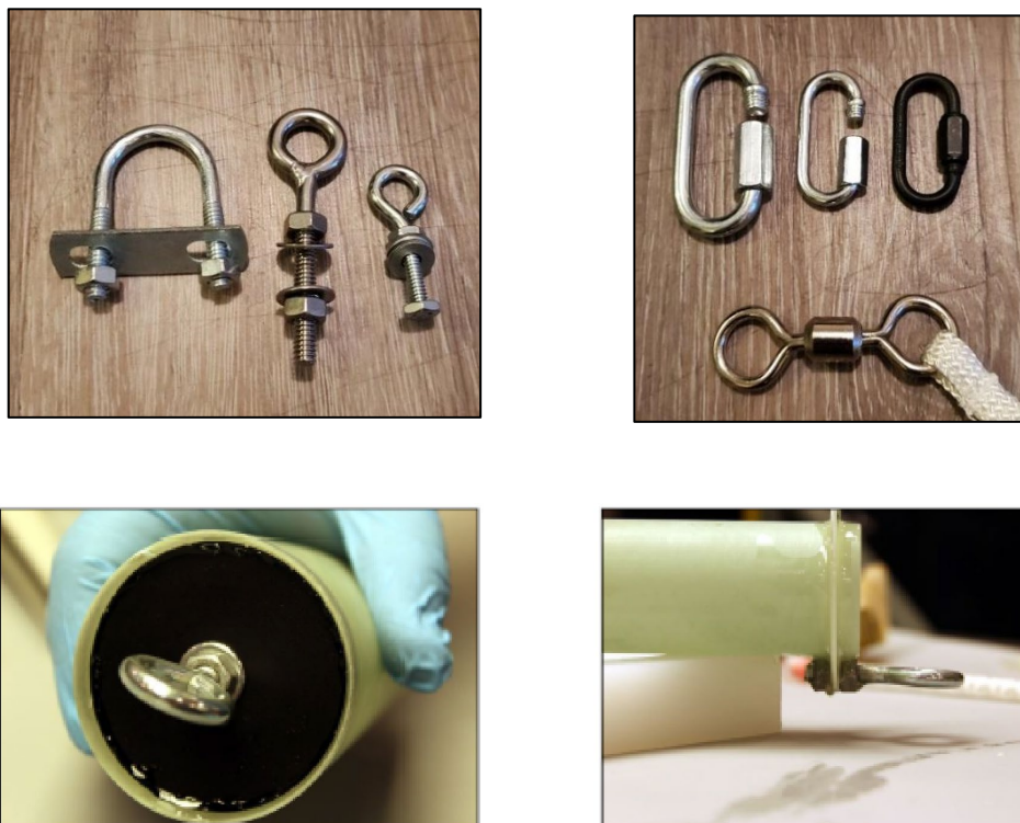
Figure 8-11: U-Bolts and Eyebolts (Upper Left); Quicklinks (Upper Left); Closed Eyebolts (Bottom)
