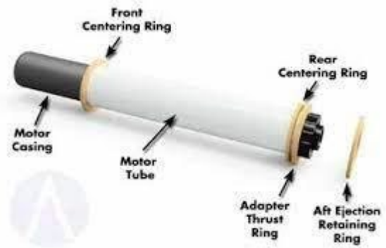
Figure 14-10: Motor Installation
