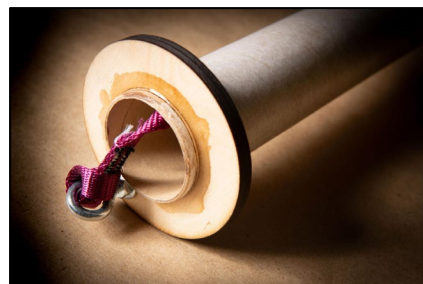
Figure 13-21: Shock Cord Installed Inside Motor Mount Tube Using Eyebolt (Left) and Quicklink and Eyebolt (Right)
