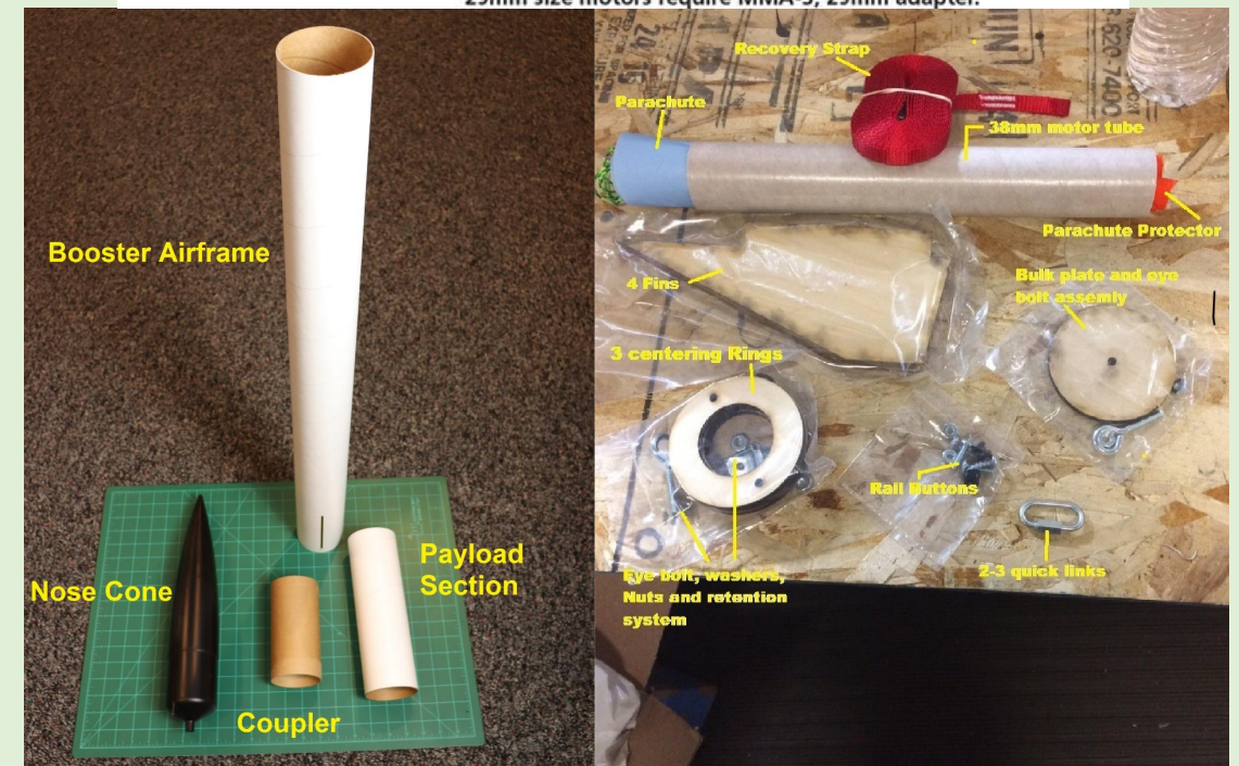
Figure 2-1: Parts included with the LOC Precision – 3.10" Caliber ISP Rocket Kit (not including parts supplied by WSGC)
