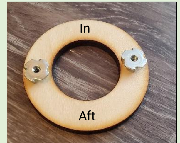
Figure 13-4: Aft Centering Ring with T-Nuts Installed
