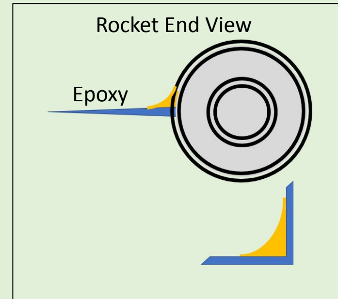
Figure 13-14: Epoxy Fillets
