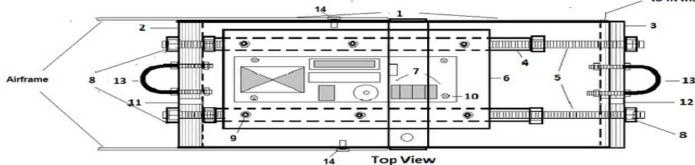
Top View
